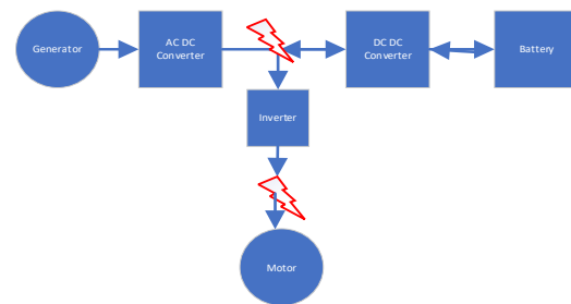
eVTOL simplified sample Electrical network
