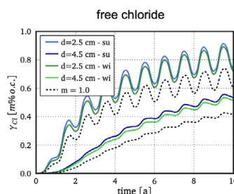
below: Chloride concentration at the column base of a parking deck.
