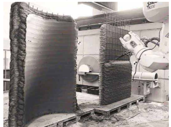
Reuse: Reinforced large-scale concrete components are digitally manufactured in a combined process of SC3DP core printing, vertical cover layer printing and precise surface finishing by CNC milling
