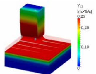
below: Chloride concentration at the column base of a parking deck.
